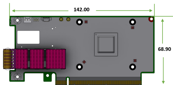
Single-Port QSFP56 x16 Adapter Cards Mechanical Drawing
