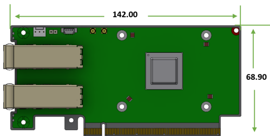
Dual-Port SFP28/SFP56 x16 Adapter Cards Mechanical Drawing
