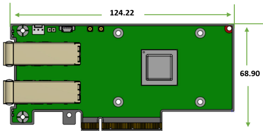
Dual-Port SFP28/SFP56 x8 Adapter Cards Mechanical Drawing
