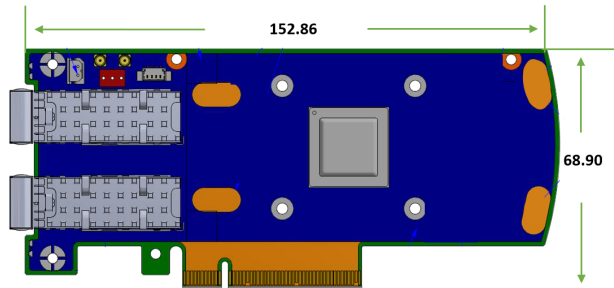
Dual-Port SFP28 x8 Adapter Cards with Active Cooling Mechanical Drawing
